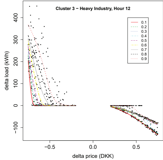
Fig. 2. Flexibility of 210 heavy industry customers in cluster 3. The graph shows hour 12 with 9 quantile regressions.
